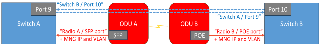
Figure 58: LLDP flow
