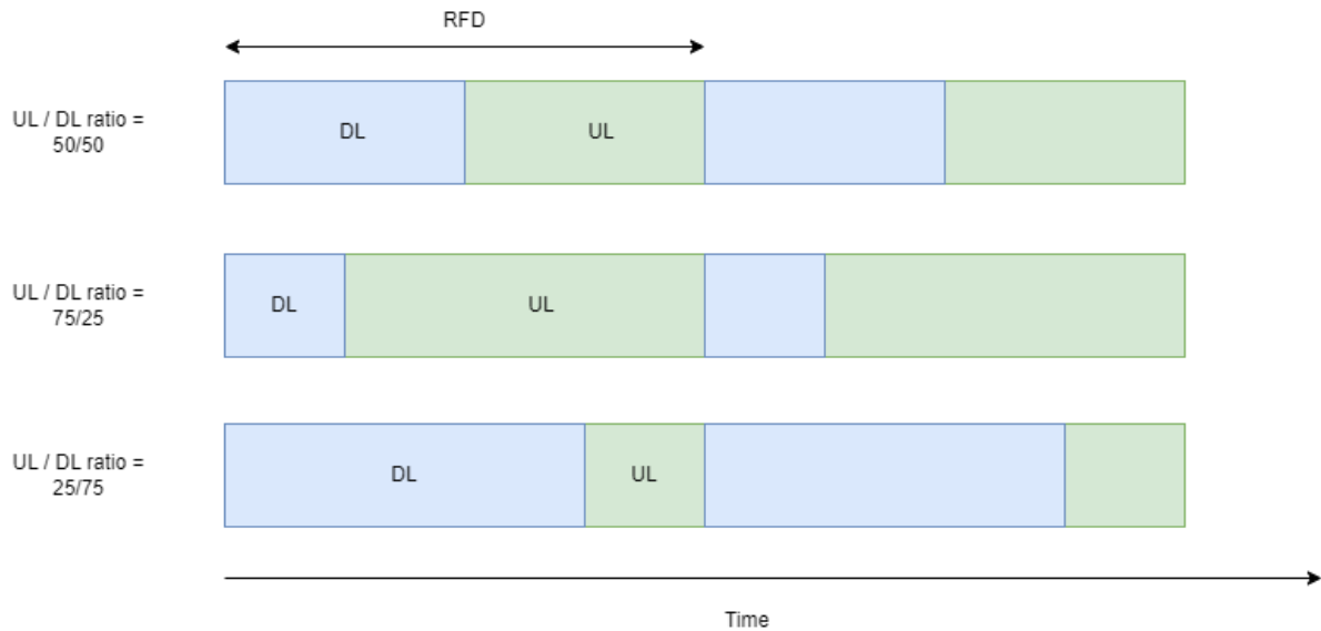
Figure 6: TDD ratio
